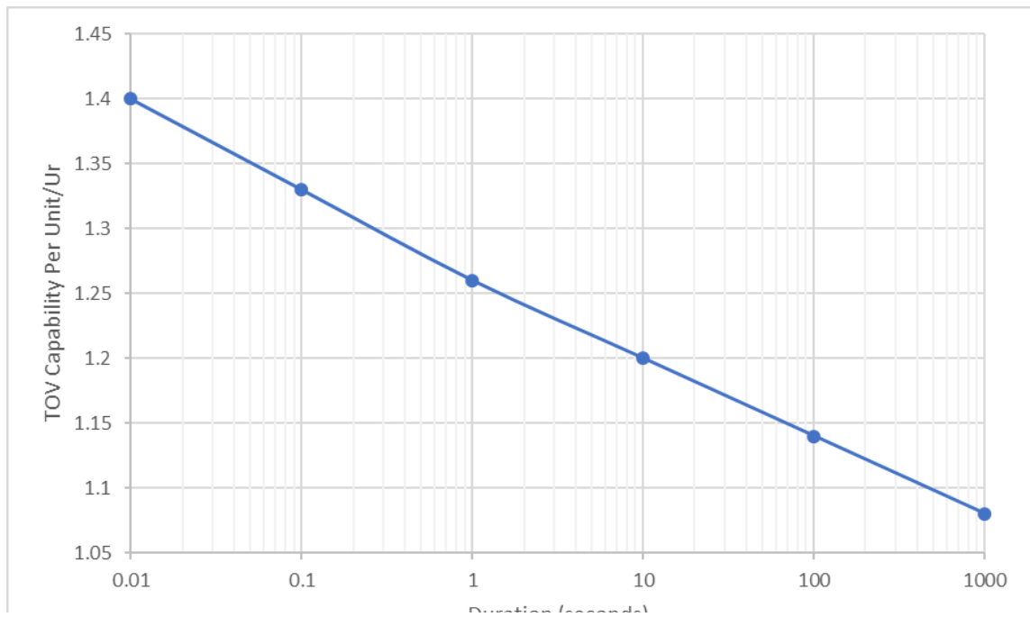
Figure 1: TOV Capability (without capacitive ground lead disconnecter bracket)
